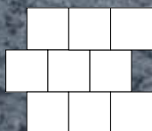
Brickwork Square / Diamond Pattern Size/Qty per sm 300x300 / 11.111 600x600 / 2.778 900x900 / 1.235
